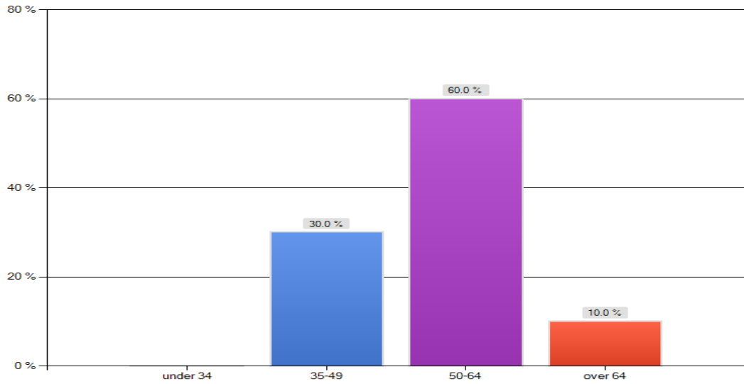
Figure 15: Survey Question Twenty
